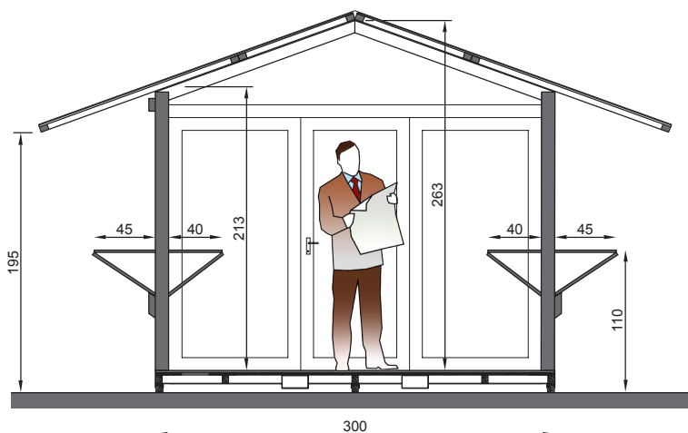
front section
