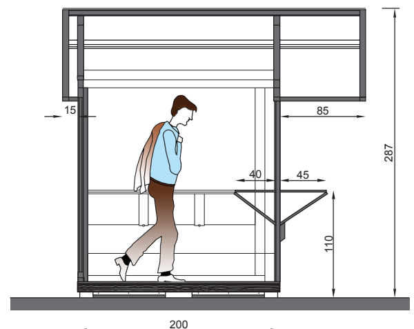
side section
